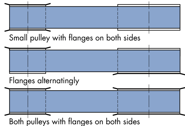
Figure 7.3.3: Arrangement of the flanges on a two-pulley drive
