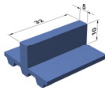
Figure 6.4.5: Dimensioned cleat
