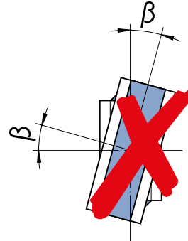
Figure 7.7.3: Parallel alignment, type of fault: Interleaving
