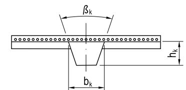
Figure 1.4.8: ATK profile with notched V-guide in cross profile
