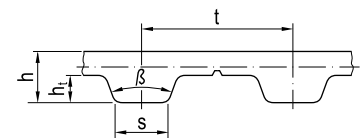
Figure 1.4.1: Imperial profile
