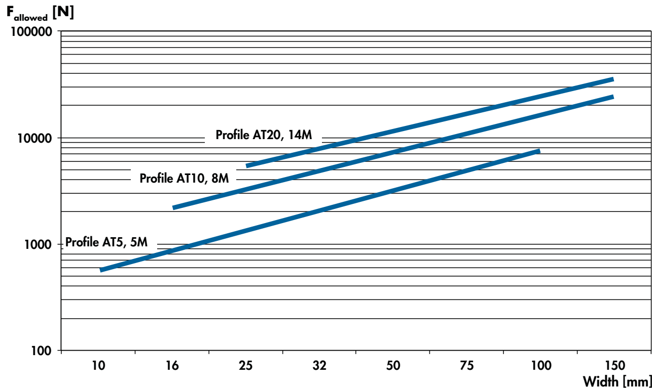
Diagram 4.3.2: AT and HTD profile, permissible tensile forces F_{\text{allowed}} depending on profile and width in a simplified representation
