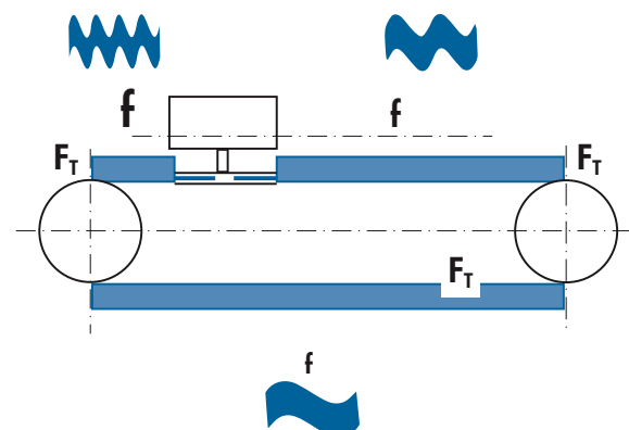
Figure 4.5.2: Frequency f depending on static belt tension F_T and span length L
